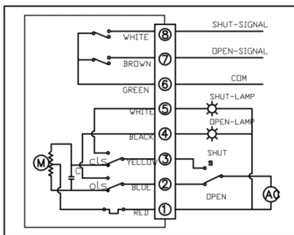
AC220V
