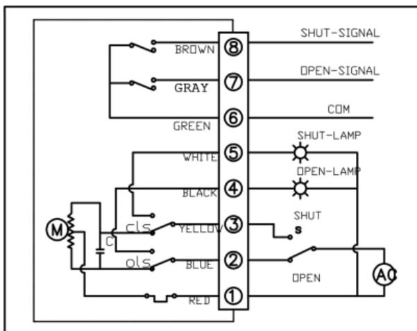
AC220V
