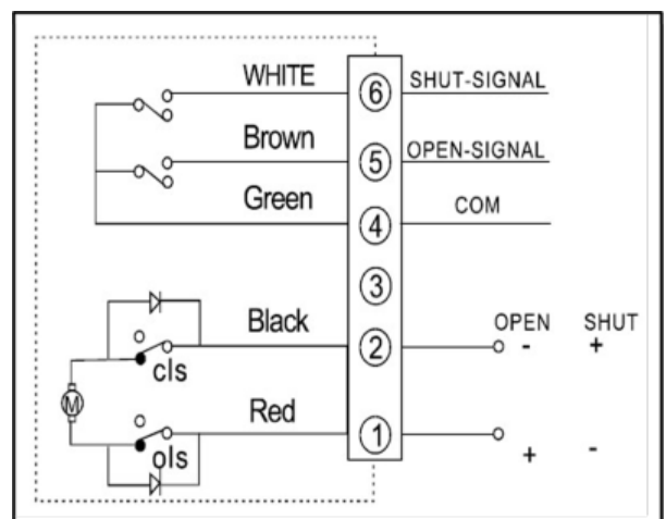
DC24V
