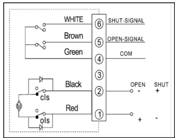
DC24V
