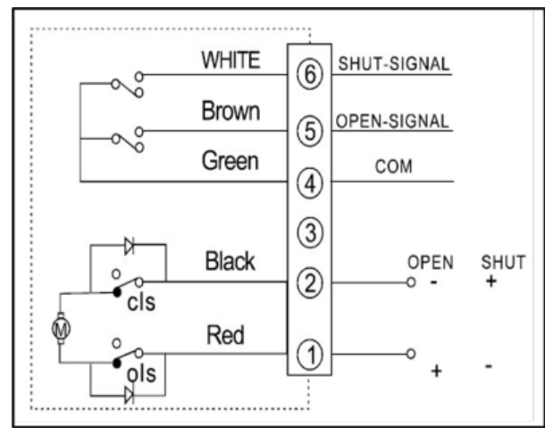
DC24V
